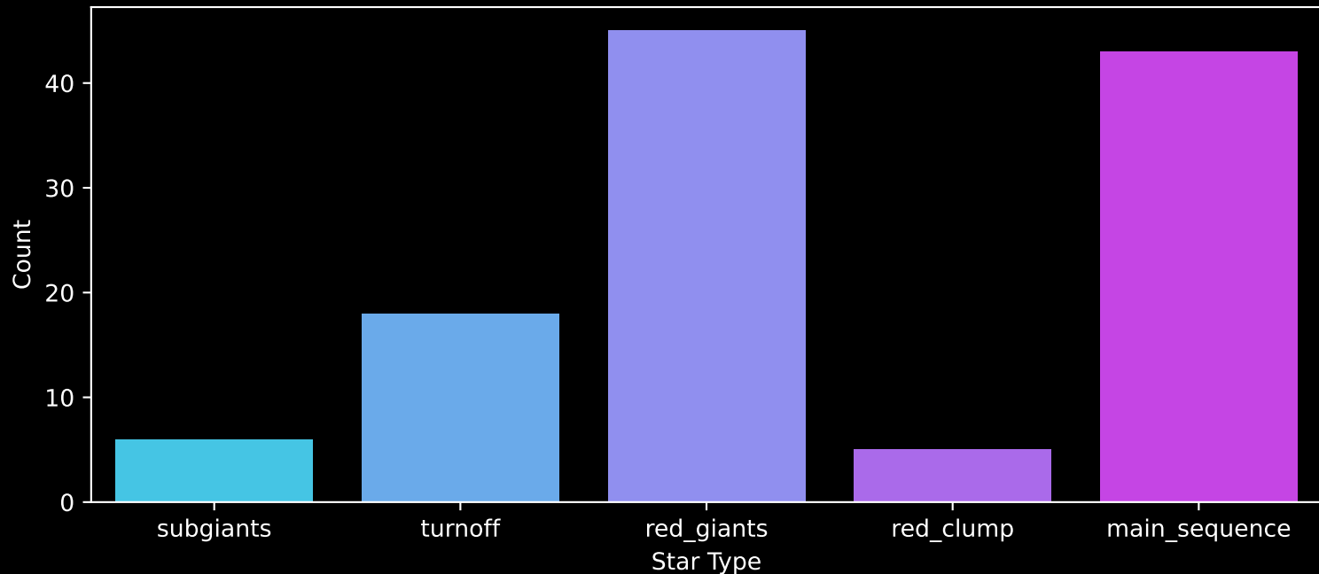
APOGEE DR17 Field: [005+02-O] Count plot of Star Type
