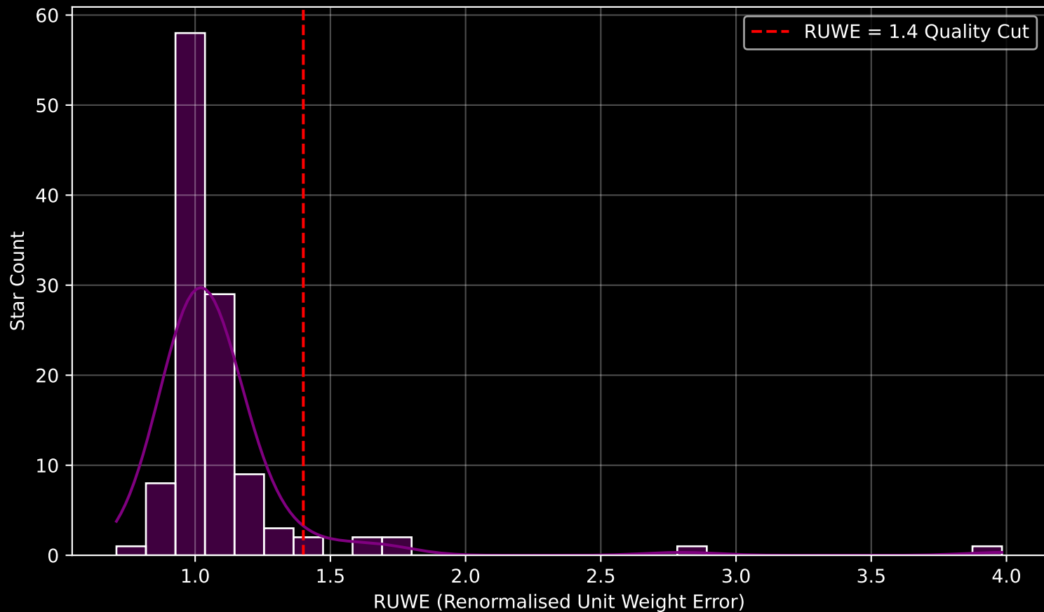
GAPOGEE DR17 Field [005+02-O] RUWE Distribution (n= 116)
