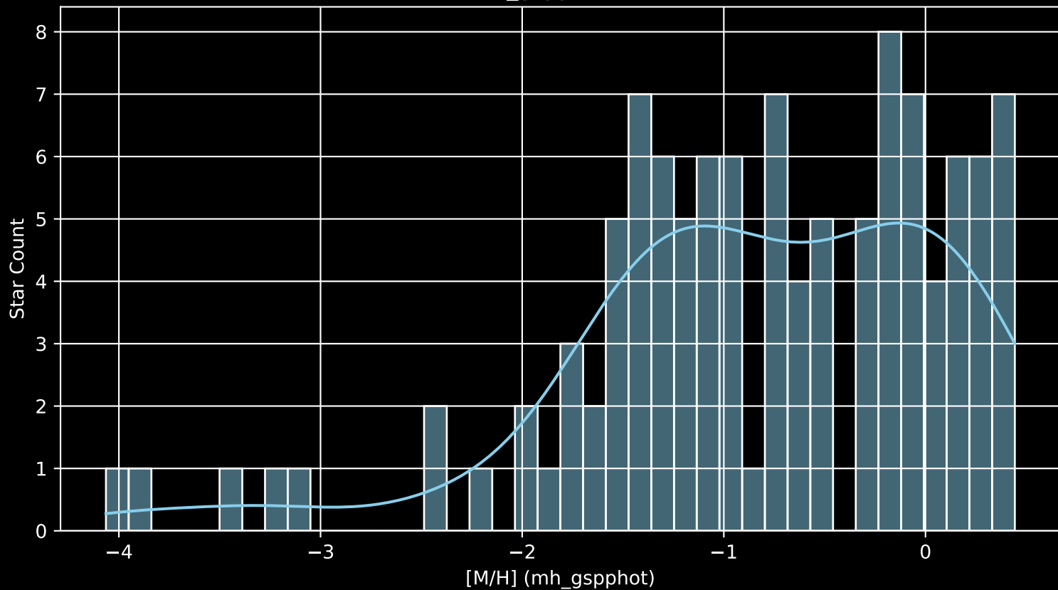
APOGEE DR17 Field: [005+02-O [M/H] (mh_gspphot) (n= 111)
