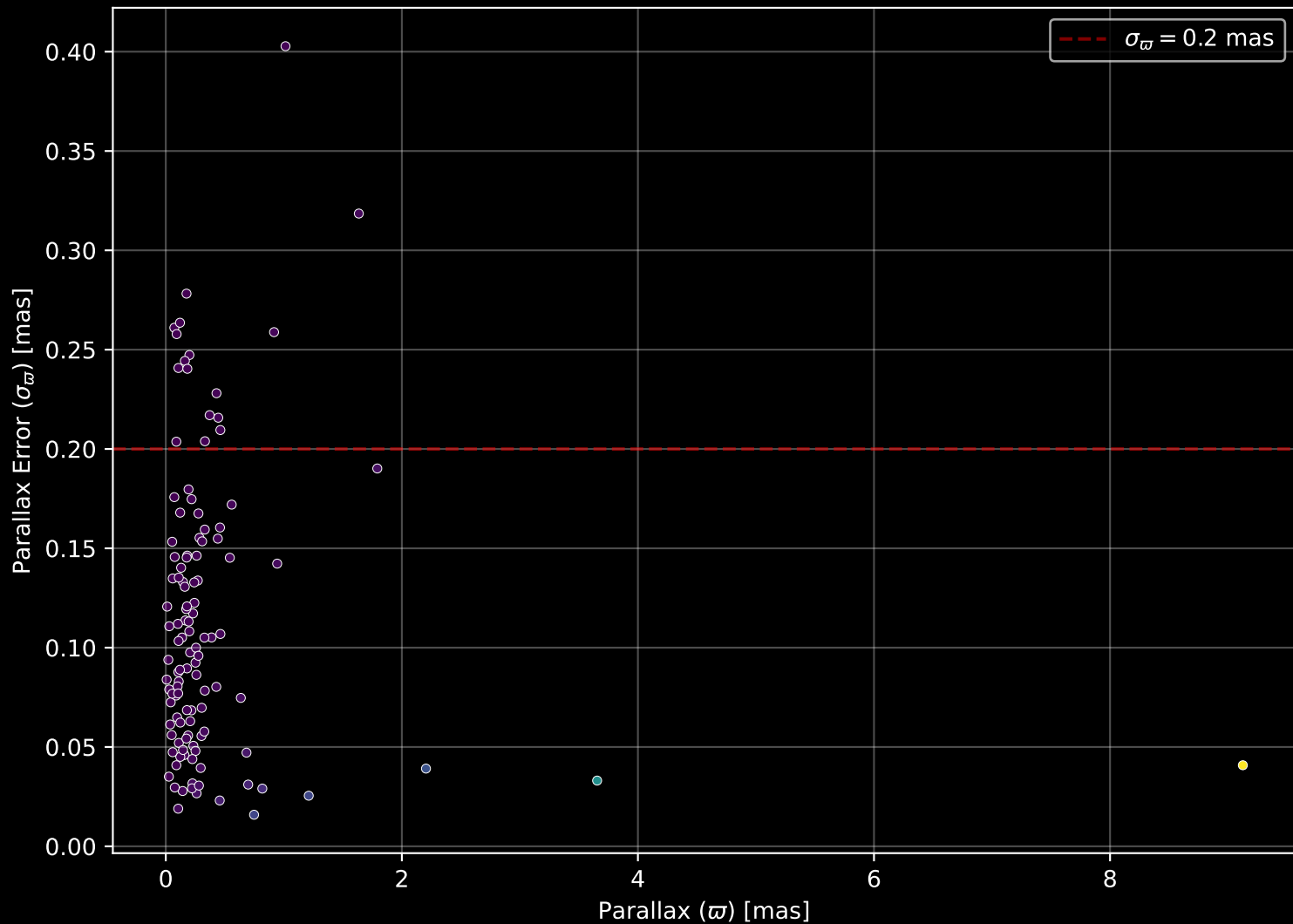
APOGEE DR17 Field: [005+02-O] Parallax Quality (n= 117)
