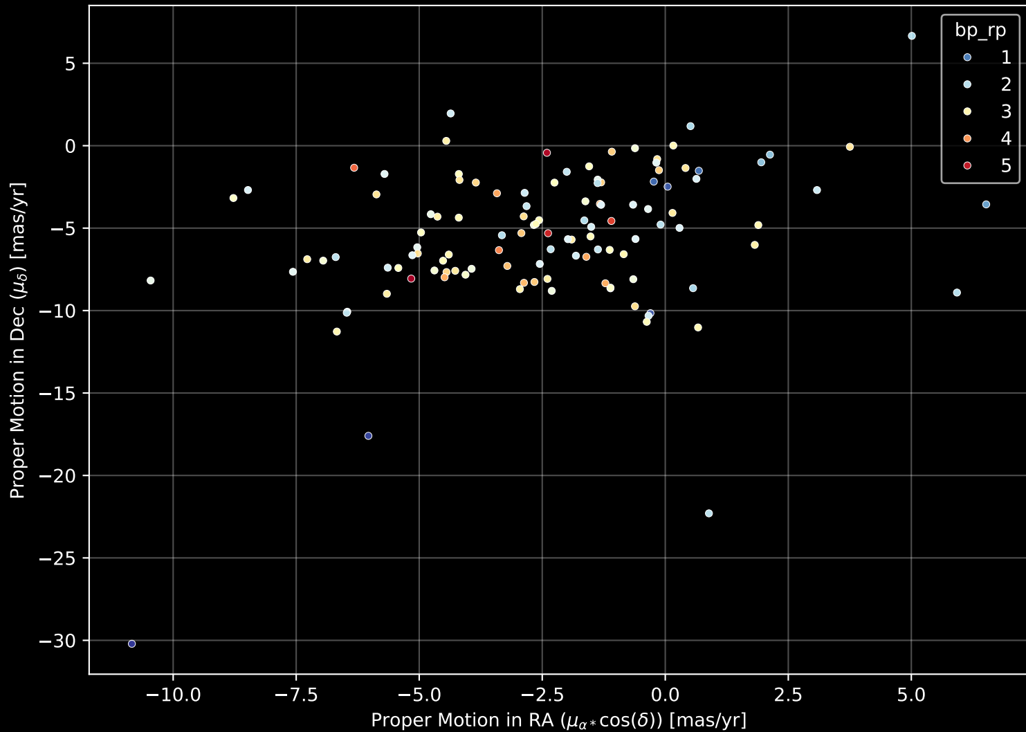
APOGEE DR17 Field: [005+02-O] Proper Motion Diagram (n= 117)
